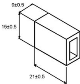
Base dimensions for Type B/Bf and I
